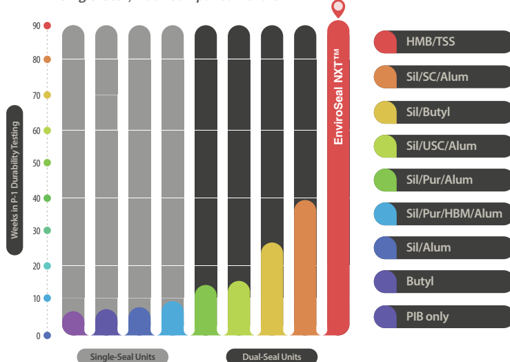
Single Seal, Dual Comparison Chart 125+ Weeks
